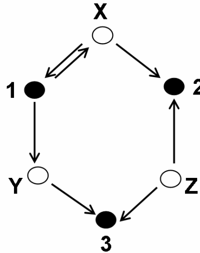
Scheme 2. Two representations of a oscillophore of minimum size. Open circles correspond to molecular species, filled circles correspond to processes, including exit from the system
